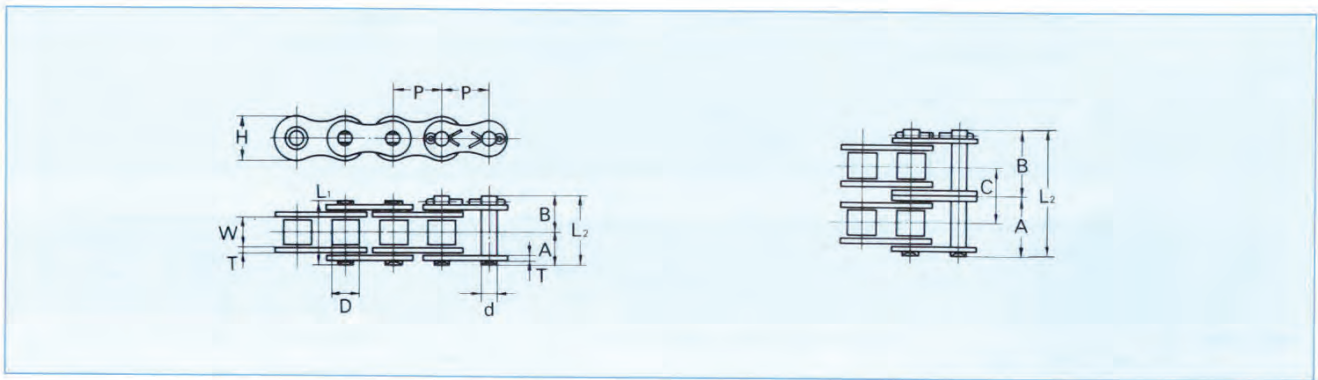
Dimensions (millimeters)
