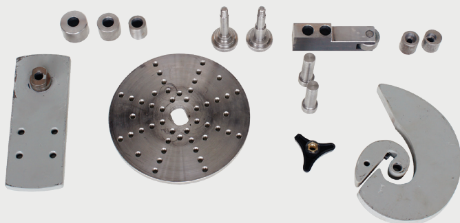
Wrought Iron Bender Attachment Components
