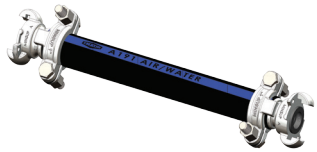
1" (DN25) Black Minsup assembly with claw clamps
