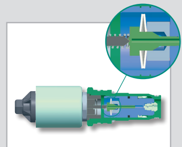
Control valve
