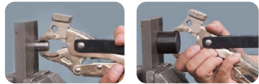
SELF ALIGNING PULL BAR
