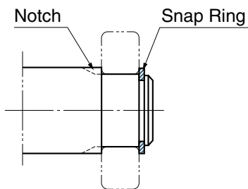
Fig. 8.13 (a) Snap Ring and Notched Shoulder
