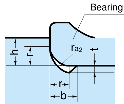
Fig. 8.8 Chamfer Dimension and Radius of Corner Roundness
