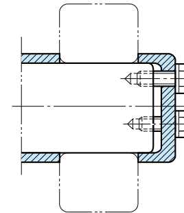
(c) End Plate and Bolts
