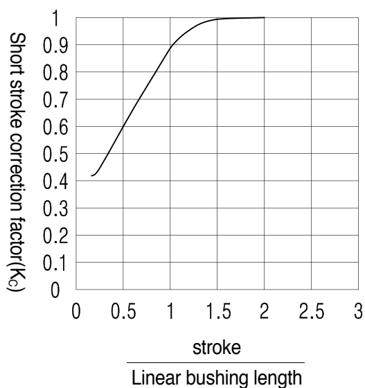
Fig 5. Short stroke correction factor( K_c )
