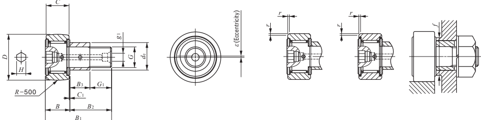
CFE...BR Outside diameter of eccentric collar d_e 16-41mm
