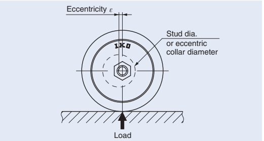
Fig. 5 Reference position for adjusting of Solid Eccentric Stud Type Cam Followers and Eccentric Type Cam Followers
