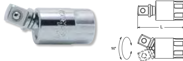
2771 Universal Joint
