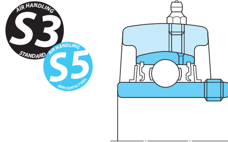
Fig. 2.3 Structure of bearing units for blowers
