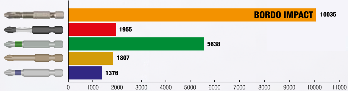
PH2x50MM CYCLES BEFORE FAILURE average impact 10.3 Nm at 100% loading
