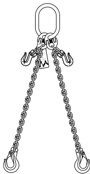
2 Leg Chain Sling Grab & Sling hook
