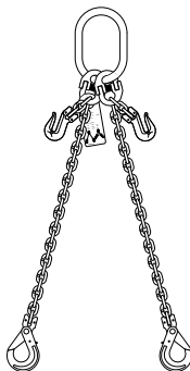
2 Leg Chain Sling Grab & Self lock hook
