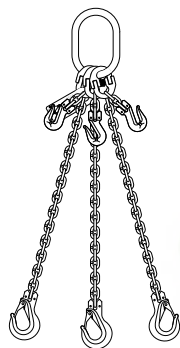
3 Leg Chain Sling Grab & Sling hook
