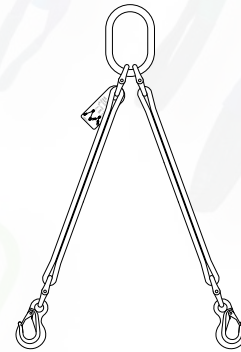
2 Leg Round Sling Sling hook
