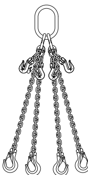
4 Leg Chain Sling Grab & Sling hook
